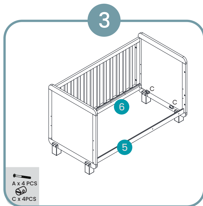
Assemble the mattress side using 4 x A bolts with 4 x C nuts
