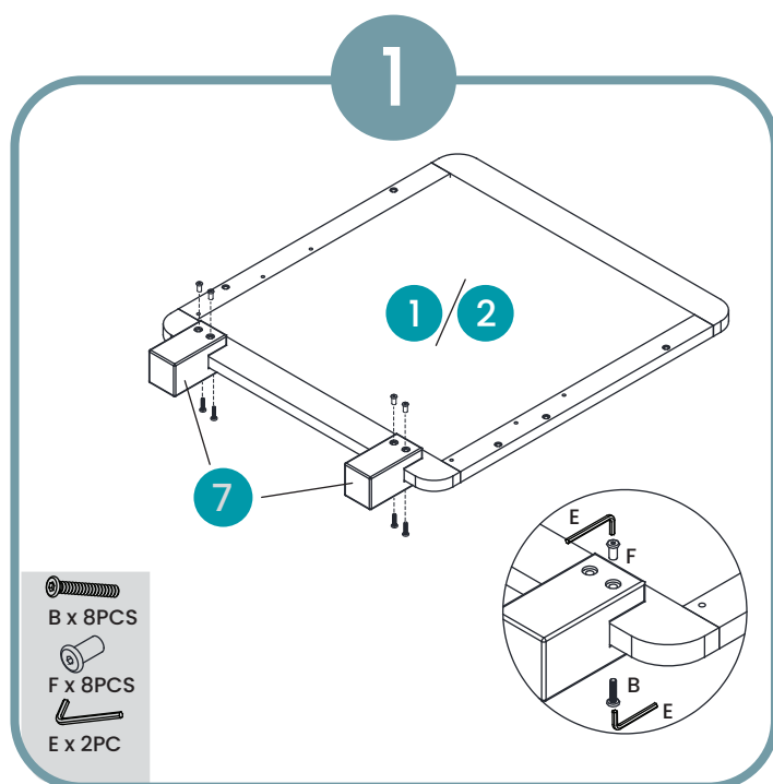
Assemble foot using 8 x B bolts with 8 x F nuts
