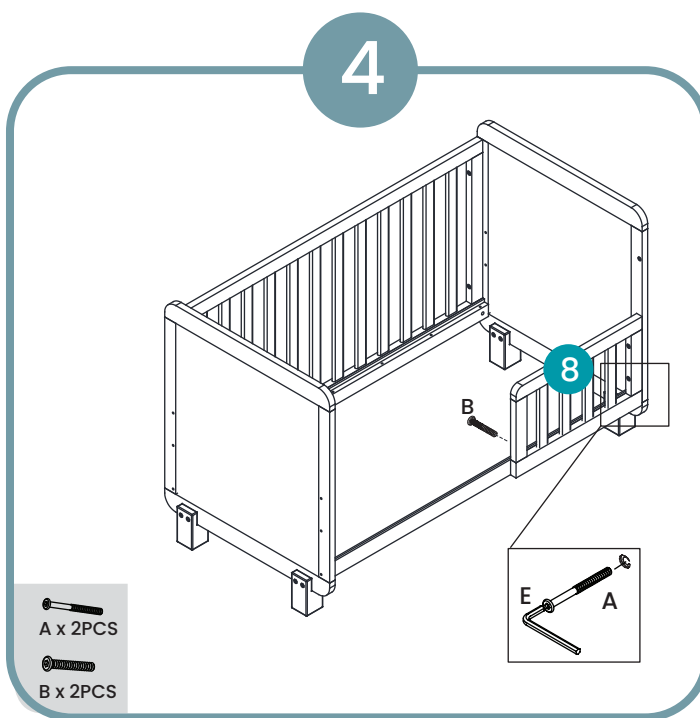
Assemble small side using 2 x A bolts with 2 x B bolts
